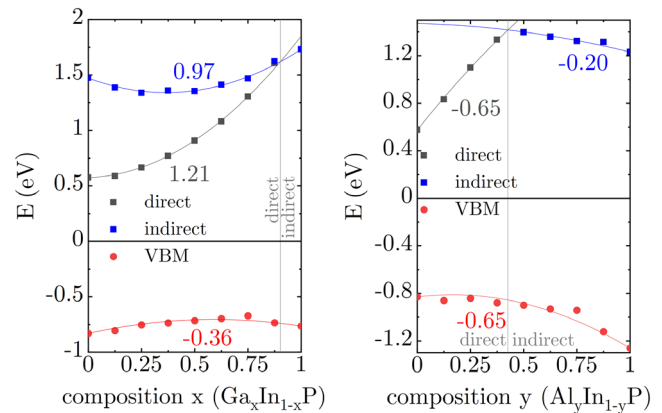
Figure 2. Composition dependence of branch-point aligned valence and conduction band energies of \text{Ga}_x\text{In}_{1-x}\text{P} (lhs) and \text{Al}_y\text{In}_{1-y}\text{P} (rhs) calculated within hybrid DFT. The solid lines result from fits to Equation (2). The bowing parameters (in eV) as well as the direct–indirect crossover compositions are indicated.
