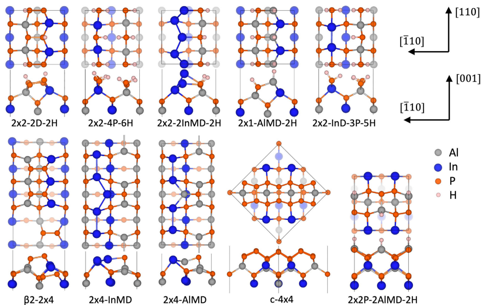
Figure 2. Top and side views of stable relaxed clean as well as hydrogenated Al_{0.5}In_{0.5}P(001) surface structures identified in the present work.
