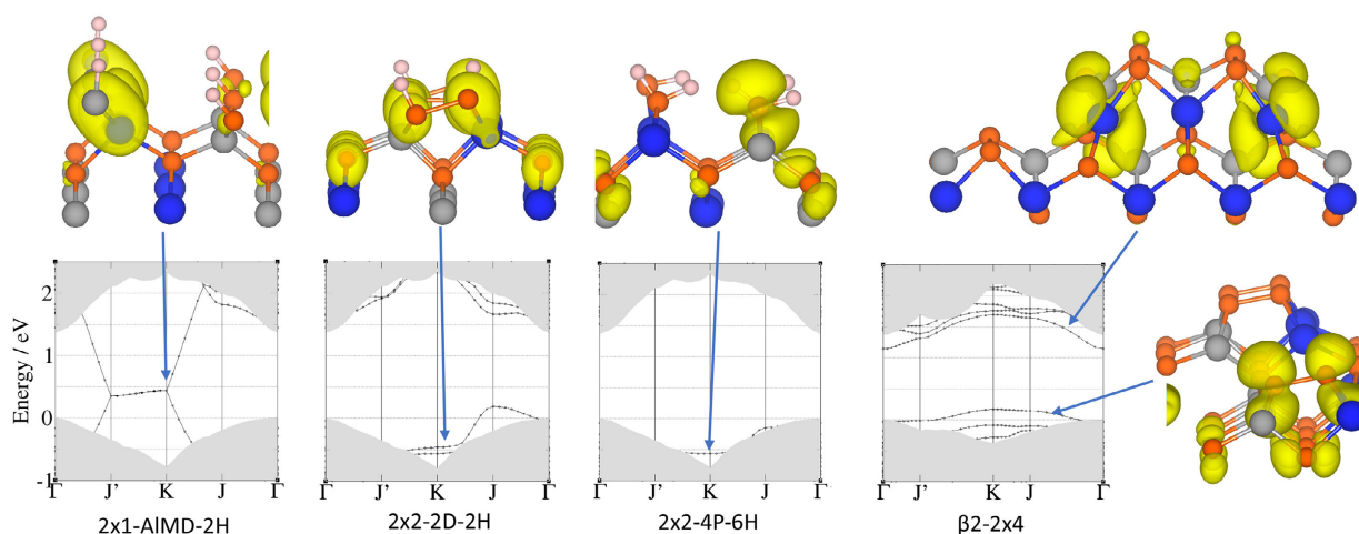
Figure 5. Band structures of the thermodynamically most relevant surface structures as well as of the 2 \times 1\text{-AlMD-}2\text{H} surface. Gray regions indicate the projected bulk band structure. \Gamma and \Gamma' are parallel to \bar{1}10 and \bar{1}10 , respectively. The orbital character of state (at the K point) is indicated for prominent surface states. See Figure 2 for notation of atoms.
