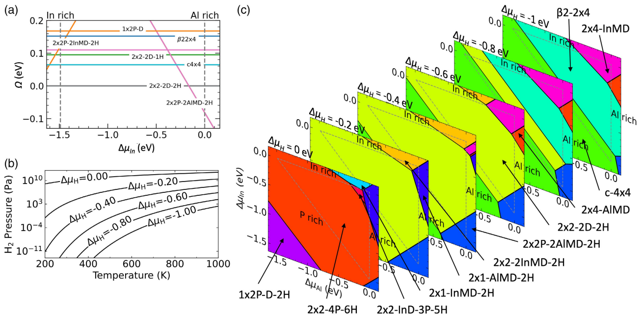
Figure 1. a) Al_{0.5}In_{0.5}P(001) surface phase diagram calculated assuming P-rich surfaces and \Delta\mu_H = -0.6 eV, that is, preparation conditions typical for vapor-phase epitaxy. Energies are given relative to the 2 \times 2 -2D-2H surface. b) Dependence of the hydrogen chemical potential on temperature and partial pressure according to Equation (4). c) Complete surface phase diagram depending on the Al, In, and H chemical potentials. The thermodynamically allowed range of the chemical potentials according to Equation (2) and (3) is indicated by dashed lines. See Figure 2 for the notation of surface structures.
