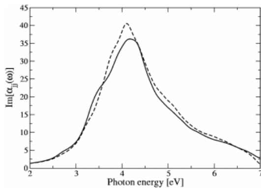
Fig. 10 Imaginary part of the slab polarizability (2) of Si(001) 2 \times 1 -H for two directions of the light polarizations. Solid line: j \equiv x , dashed line: j \equiv y . The calculations were performed including quasiparticle, LF and electron–hole attraction effects.
