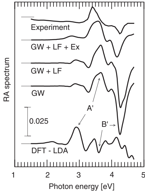
Fig. 9 RA spectrum calculated in different approximations with respect to the many-body effects for the monohydride Si(001) 2 \times 1 -H surface [57]: within DFT-LDA (i.e., using KS eigenvalues \varepsilon_v(\mathbf{k}) ); in the GW approximation (i.e., shifted by quasiparticle shifts (9)); in the GWA with LF effects (i.e., \bar{v} (7) is included in the Hamiltonian (5)), and in the GWA with LF effects and screened electron–hole attraction (i.e., the interactions \bar{v} (7) and W (6) are fully included in the Hamiltonian (5)). The computed spectra are compared with measured data (i.e., experiment) [26].
