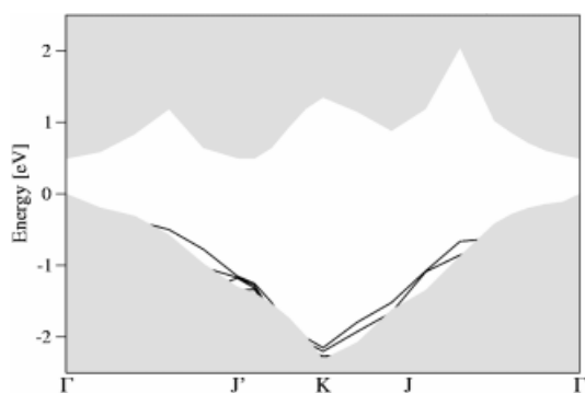
Fig. 8 Band structure of the Si(001)2 × 1–H surface in DFT-LDA quality. Grey regions indicate the projected bulk band structure.
