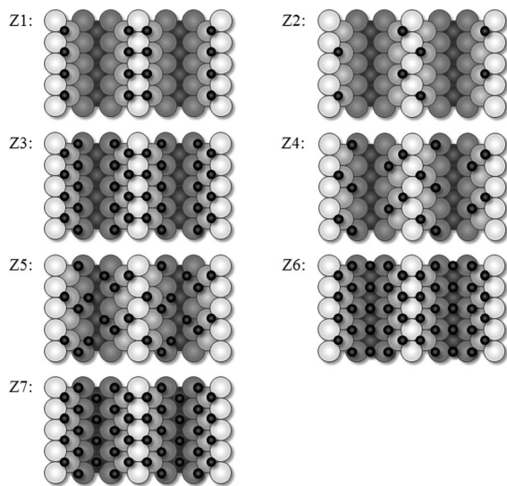
Figure 4. Schematic top views of the considered arrangements of oxygen atoms (black colored circles) on the Au(110)-(1 × 3) surface. Darker gray colored circles indicate gold atoms in deeper atomic layers.
