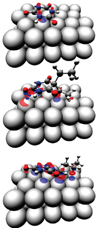
Figure 2. Adsorption geometries for CYA, DEB and BuCYA at Au(111). Charge accumulations are marked in blue, depletions in red (iso-surface value: 0.005 \text{ e}/\text{\AA}^3 ).
