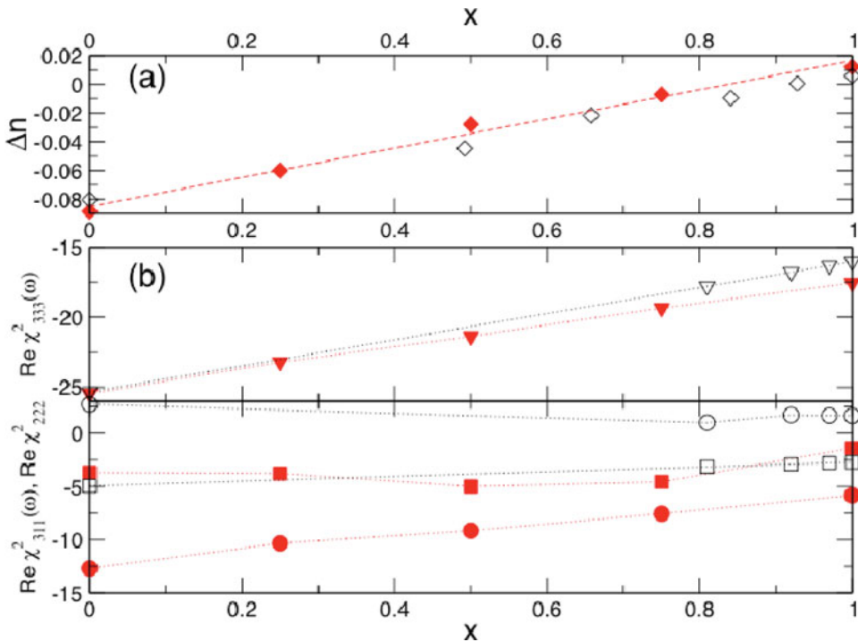
Figure 5. (a) Calculated birefringence \Delta n (filled diamonds) for LiNb 1-x Ta x O 3 for \lambda = 632.8 nm (1.96 eV). Hollow diamonds denote experimental values obtained by Wood et al. [2]. (b) Nonlinear coefficients \chi^{(2)}_{333} , \chi^{(2)}_{311} , and \chi^{(2)}_{222} (in pm/V) for \lambda = 1.064 \mu\text{m} (1.17 eV) calculated within the IPA (filled triangles, squares, and circles) compared with results from semi-empirical calculations by Xue et al. [3] (hollow symbols). Dotted lines are to guide the eyes (Color figure available online).
