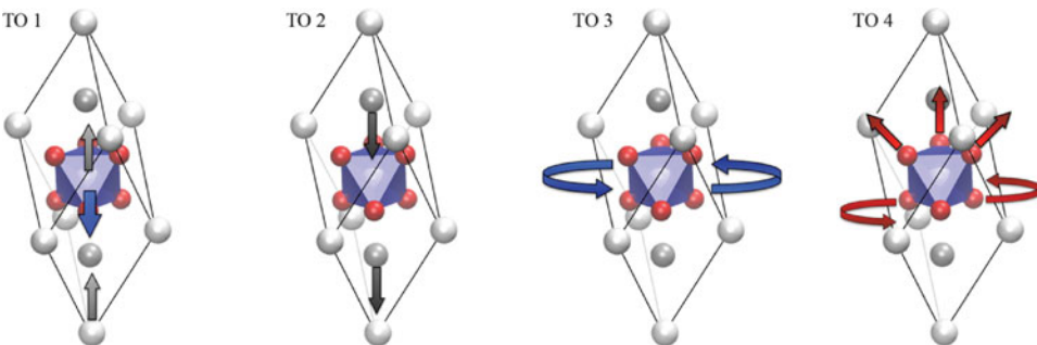
Figure 2. Eigenvectors of the four vibrational transversal branches (TO1 to TO4) of \text{LiNbO}_3 and \text{LiTaO}_3 . Arrows represent schematically the displacement patterns (see text for further details).
