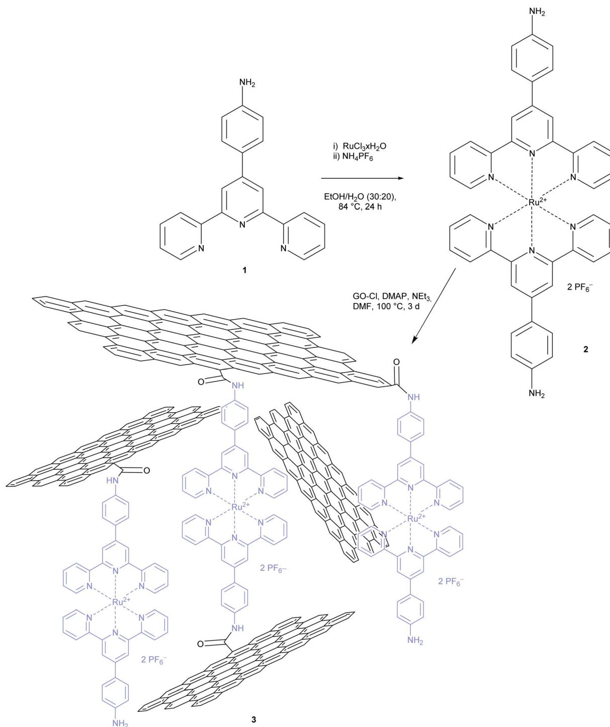
Scheme 1 Synthesis of [Ru(bis-terpyridine)] complex 2 and functionalized GO material 3.
