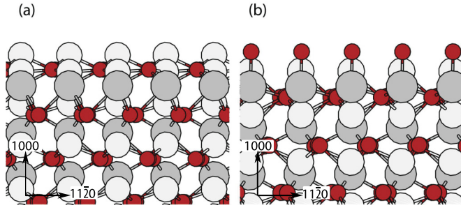
FIG. 1. (Color online) Side view of the stable positive (a) (-Nb-O 3 -Li 2 terminated) and negative (b) (O-Li- terminated) LN(0001) surface. White, gray, and small circles denote Li, Nb, and O atoms, respectively.
