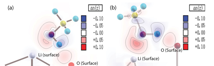
FIG. 5. (Color online) Calculated charge-density difference (in e/\text{\AA}^3 ) of the methanol bonding configuration A on the positive (a) and negative (b) LN surface.
