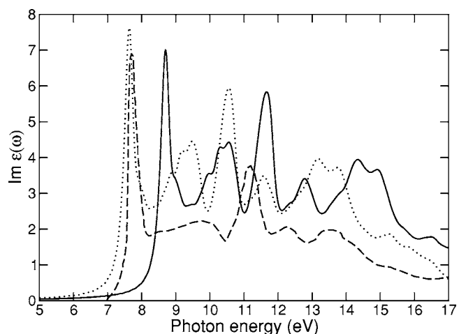
FIG. 7. Imaginary parts of the macroscopic dielectric function calculated including quasiparticle and excitonic effects without (solid line) and with (dotted line) the effect of the lattice polarization for rs -NaCl. The experimental room-temperature spectrum (Ref. 29) is shown as dashed line. A Lorentzian broadening of 0.2 eV has been used.
