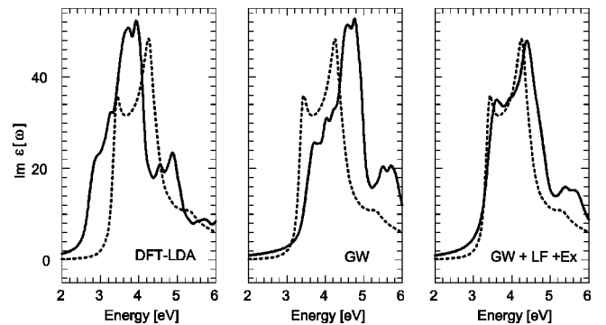
FIG. 3. Dielectric function (imaginary part) of bulk Si calculated within the DFT-LDA, in GW approximation, and from the BSE (GW + LF and excitonic effects) in comparison with the experimental data from Ref. 33 (dotted line).
