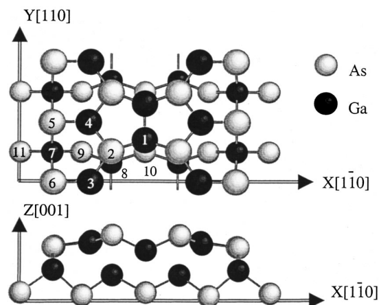
FIG. 1. Ball and stick model of the \zeta(4 \times 2) unit cell, as proposed in Ref. 8.
