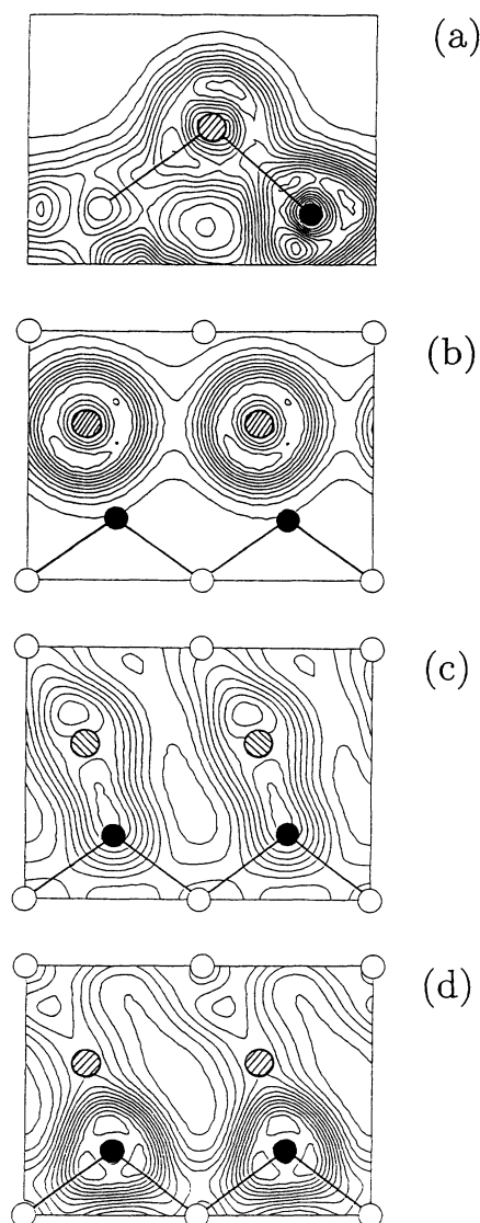
FIG. 9. Contour plot of the total valence-pseudocharge density for the system Sb/GaAs(110) 1\times 1 with (\Theta = \frac{1}{2}) . In (a) the upper panel, the density is plotted along a plane vertical to the surface containing the bonds from the adatom to both the As and Ga atoms. In the lower panels the density is drawn along (b) (110) planes 0.6 Å above, (c) 0.5 Å below, and (d) 1.1 Å below the Sb adatom cores. The contours are spaced by 0.005 bohr -3 .
