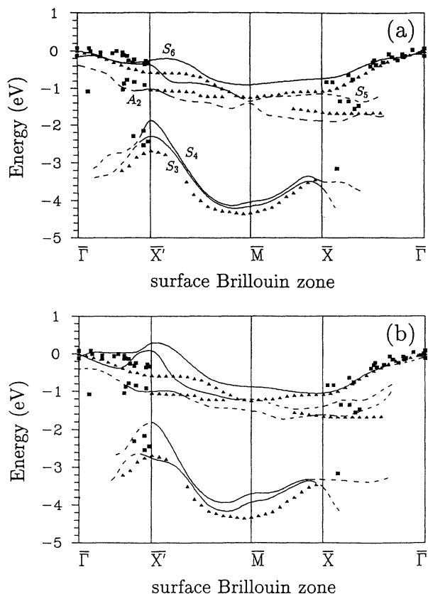
FIG. 6. Comparison of the dispersion of surface bands for Sb/GaAs(110)1×1 ( \Theta=1 ) computed for (a) ECLS and (b) EOTS models with ARPES values of Refs. 21, 22 (squares), and 23 (triangles). Solid lines indicate bound states whereas dashed lines denote resonance states. The theoretical and experimental values are aligned at the highest occupied surface state at 0 eV at \bar{\Gamma} .
