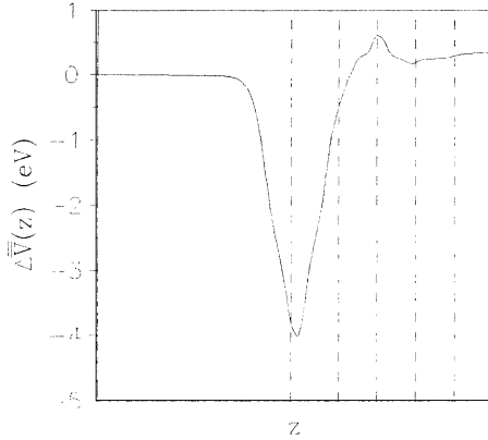
FIG. 7. Difference of the averaged electrostatic potential \Delta\bar{V}(z) for 1 ML Sb/GaAs(110) (ECLS) and the clean relaxed GaAs(110)1×1 surface versus the coordinate perpendicular to the surface. Dashed lines mark the averaged positions of the Sb and GaAs layers, respectively.
