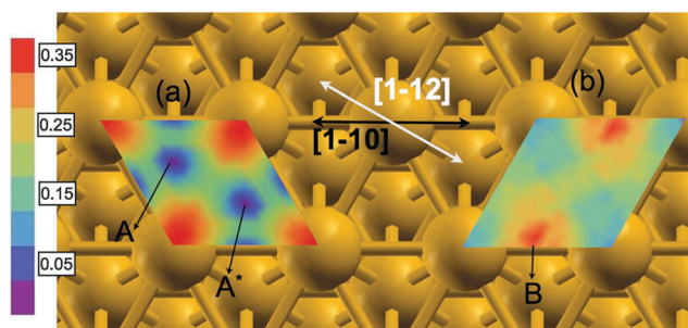
Fig. 3 The calculated PESs for single DIP molecules on Cu(111). The molecule was moved laterally and the LA was kept parallel to the (a) [112] and (b) [110] directions of the surface. The energetically most favoured structure is considered as the zero point on the scale (in eV). The most favorable hollow site A with the equivalent A* site are shown.
