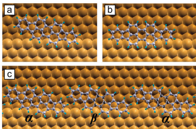
Fig. 8 Ball-and-stick representation of single DIP molecules at the Cu(111) step edges in the so-called (a) D6 and (b) E0 structures. (c) One row of molecules is shown. The molecules are arranged in incommensurable structures, where each one contains \alpha and \beta molecules.
