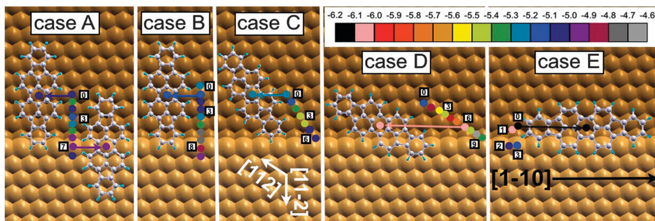
Fig. 7 Calculated adsorption geometries of DIP molecules at step edges. In case A and B, the molecular long axis (LA) is perpendicular to the step edge and parallel to the [1\bar{1}2] direction of the lower surface. The molecule binds to one atom (two atoms) of the step edge in case A (case B). In case C (case D), the LA is tilted with respect to the step edge and it is oriented along the high symmetry [101] ( [112] ) direction of the surface. In case E, the LA is parallel to the step-edge direction. For each case, a variety of registries with respect to the lower terrace have been tested. The center of the molecule is used as reference. The energies of the different structures are denoted as colored circles according to the energy scale on the upper panel. The atomic vdW-radius has been used for the Cu atoms. The upper terraces atoms have slightly lighter colors and some examples of the structures such as A0, A7, B1, C0, D6 and E0) have been depicted in detail.
