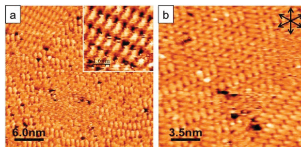
Fig. 5 STM images of DIP on Cu(111) for a submonolayer coverage, showing coexistence of LR ordered domains, SR order and a two-dimensional gas of mobile disordered molecules. (a) I = 370 \text{ pA} , bias = -0.37 \text{ V} and (b) I = 130 \text{ pA} , bias = -1.25 \text{ V} . The \langle 110 \rangle substrate directions are indicated by black arrows, while gray arrows indicate the lattice vectors of the LR ordered domains.
