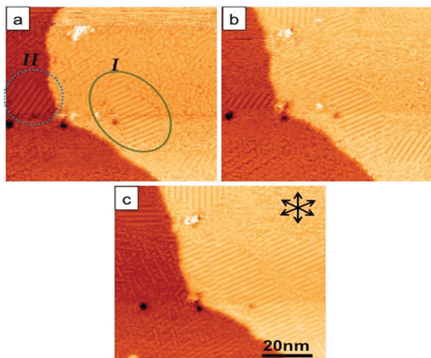
Fig. 6 (a)–(c) STM images acquired by continuous scanning in the same area ( I = 90 pA, bias = -0.45 V). (a) The LR ordered domain I is circled with a green continuous line, while domain II is circled with dotted blue line (see text for details). (b), (c) Consecutive tip scanning causes an increase of long-ranged ordering of I-type domains and the disappearance of the domain II.
