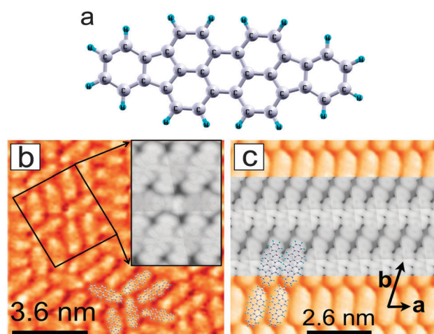
Fig. 1 (a) Ball-and-stick model of the DIP molecule. (b) The short-range (SR) and (c) the long-range (LR) arrangements of DIP molecules on Cu(111) terraces of different widths as observed experimentally using STM (cf. ref. 18). Shown in gray are simulated STM images that were obtained using the Tersoff–Hamann model (cf. ref. 30). Ball-and-stick models of DIP molecules illustrate the molecular positions on the substrate.
