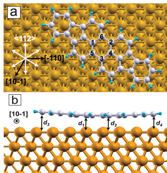
Fig. 2 (a) Top view and (b) side view of the most favored structure of single DIP molecules on Cu(111). The inner six carbon atoms are labelled from 1 to 6. The adsorption geometry is slightly concave. d_1 and d_2 denote the distances between carbon atom 1 and 2, respectively, to the Cu atoms beneath. Similarly, d_3 and d_4 denote the distances between the carbon atoms at both edges of the molecule and the Cu atoms beneath. Calculated values are given in Table 1.
