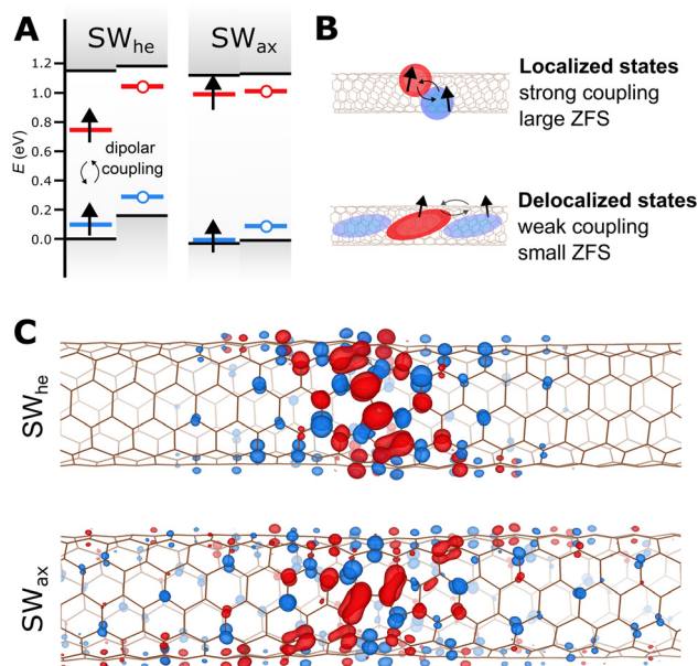
Fig. 2 (A) Schematic diagram of the DFT calculated electronic structure of the triplet ( S = 1 ; DTE) states of SW he (left) and SW ax (right). Arrows represent occupied spin-up states, while empty circles indicate unoccupied spin-down states, collectively constituting the triplet. (B) A sketch illustrating the relation between delocalization between unpaired electron and the magnitude of ZFS. (C) Partial charge density contours of the two unpaired electrons ("hole" – blue, "electron" – red) for the SW triplet DTEs. Since the unpaired electrons of SW ax are resonant with the CB and VB, they are substantially more delocalized compared to those of SW he .
