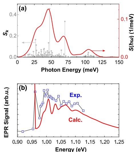
Figure 3. Electron–phonon interactions of the NV center. (A) Calculated partial Huang–Rhys factors S_k (gray) and the spectral density S(\hbar\omega) of electron–phonon coupling (red). (B) Experimental high-resolution excitation spectrum of the NV center in 3C-SiC (blue) compared with the calculated spectral function (red).
