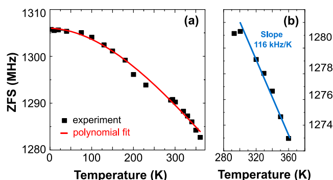
Figure 5. Temperature dependence of the ZFS parameter D . (A) Large-scale temperature variation fit with a polynomial function of order 3 (red line). (B) Temperature variation of the ZFS for T > 300 K.
