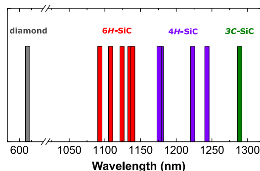
Figure 2. Overview of the NV center ZPL in diamond and in three polytypes of SiC. In diamond, the ZPL is located in the visible spectral range, whereas, in SiC, they are shifted to the telecom wavelength compatible with low-loss optical waveguides (4H-SiC data from refs 22 and 6, H data from ref 23, and 3C-SiC this work).
