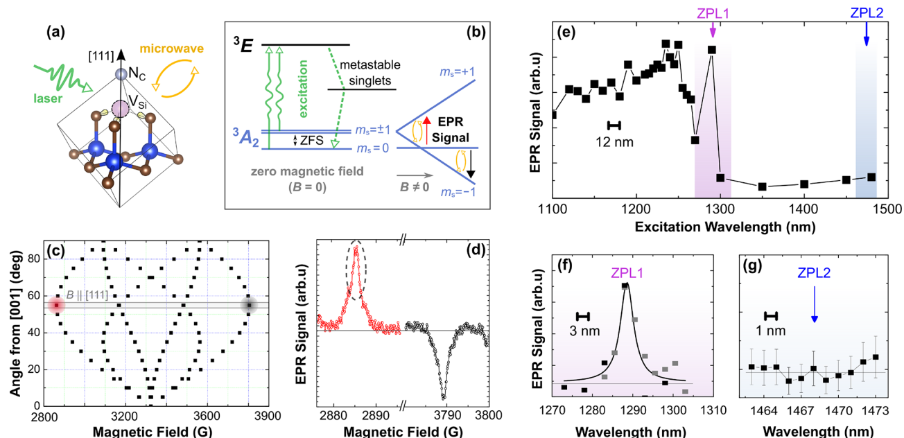
Figure 1. Resonant optical excitation experiment. (a) Schematic atomic structure of the NV center aligned with the crystallographic [111] direction of 3C-SiC. (b) energy level diagram illustrating the ground and excited states and the optically induced ground-state spin polarization. The applied magnetic field causes Zeeman splitting of ^3A_2 ; the preferential population of the m_s = 0 level will invert the phases (absorption/emission) of the low- and high-field EPR transitions |m_s = 0 \rightarrow m_s \pm 1| . (c) Angular variation of the NV center resonance fields for a rotation of the applied magnetic field in the (110) plane. The resonance fields of the [111] aligned NV center are highlighted. (d) Low-temperature ( T = 4 K) EPR spectrum of the [111] aligned NV center under resonant optical excitation. The optically induced ground-state spin polarization results in an absorption and emission line shape for the low-field and high-field lines, respectively, with a close to 100% spin polarization. The low-field EPR line at 2870 G is used for the resonant excitation measurements. (e) Large-scale excitation spectrum of the EPR signal intensity measured with a resolution of 12 nm; (f) high-resolution excitation spectra of the NV center at the ZPL1 at 1289 nm (ZPL1) and (g) the ZPL2 at 1468 nm. Only the ZPL1 is related to the NV center.
