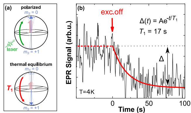
Figure 4. Decline of the ground-state spin polarization. (A) Simplified sketch of the distribution of Bloch vectors with (top) and without (bottom) resonant optical excitation illustrating the population difference between the m_s = 0 and m_s = \pm 1 ground-state spin sublevels. Without excitation, spin–lattice relaxation drives the populations toward thermodynamic equilibrium with the time constant T_1 . (B) Time-resolved EPR signal intensity at T = 4 K after switch-off of the optical excitation. The red line shows the fit with a single exponential decline with the time constant T_1 = 17 s.
