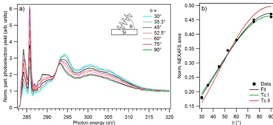
Figure 9. (a) C K-edge NEXAFS spectra (for different angles of incidence \theta ; see inset) for a nominally 1 nm-thick ultrathin Tc film at H–Si(111) grown and measured at LT. (b) \pi^* resonance intensities derived from the spectra shown in part a as a function of \theta , a fit to the data according to eq 1, and the expected curves for pure Tc I (bulk) and Tc II (thin film) crystal phases (Error bars are within the size of the symbols).
