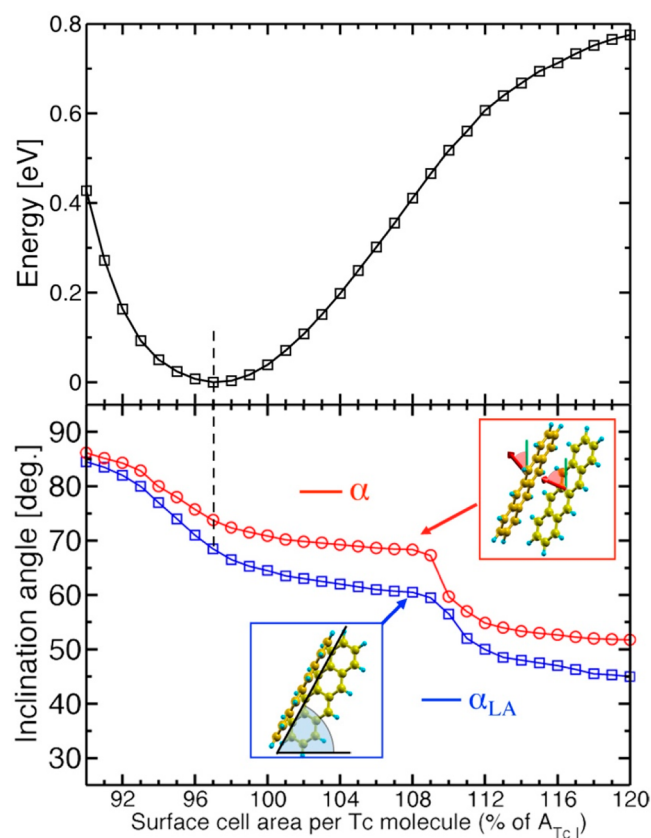
Figure 5. (top) Total energy for Tc monolayers as a function of the surface unit cell area per molecule, referenced to that of bulk-Tc ( A_{\text{Tcd}} ). The energy minimum is at 97% of A_{\text{Tcd}} , as in the case of the Tc I-type structure shown in Figure 3. (bottom) Corresponding geometric inclination angle \alpha_{\text{LA}} , defined by the average orientation of the molecules' long axis (LA) against the surface plane. Note that \alpha_{\text{LA}} is different from \alpha determined from the NEXAFS analysis, which is also included. For increasing lateral cell size to about 130%, \alpha_{\text{LA}} goes slightly down to about 40^\circ , before for even lower coverage more individual arrangements in pairs or even flat-lying molecules are preferred.
