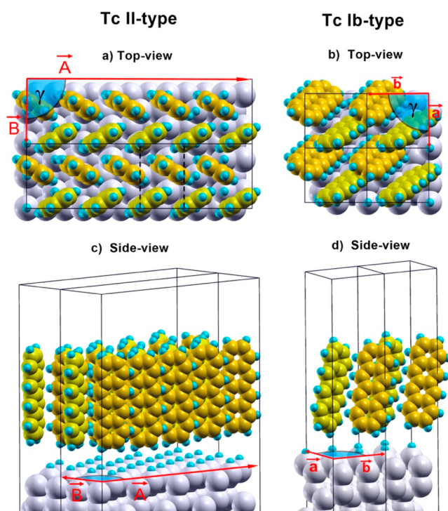
Figure 6. (a) [(b)] Top and (c) [(d)] side views of the geometries of a Tc monolayer calculated in rectangular supercells of lateral dimensions \vec{A} = 0.772 nm, \vec{B} = 2.702 nm [ \vec{a} = 0.675 nm, \vec{b} = 0.772 nm] and \gamma = 90^\circ , resembling 1 \times 5 [ 1 \times 1 ] unit cell reconstructions for Tc II-type [Tc Ib-type], respectively. These structures represent 10% more dense (Tc II-type) and 10% less dense coverage (Tc Ib-type) in comparison to the most stable Tc I-type structure shown in Figure 3. The corresponding epitaxy matrices are given by \begin{pmatrix} A_{\text{Tc II-type}} \\ B_{\text{Tc II-type}} \end{pmatrix} = \begin{pmatrix} 2 & -2 \\ 4 & 4 \end{pmatrix} \begin{pmatrix} \vec{x}_1 \\ \vec{x}_2 \end{pmatrix} and \begin{pmatrix} a_{\text{Tc Ib-type}} \\ b_{\text{Tc Ib-type}} \end{pmatrix} = \begin{pmatrix} 1 & 1 \\ 2 & -2 \end{pmatrix} \begin{pmatrix} \vec{x}_1 \\ \vec{x}_2 \end{pmatrix} , where \vec{x}_1 and \vec{x}_2 again indicate the primitive vectors of the H–Si(111) substrate.
