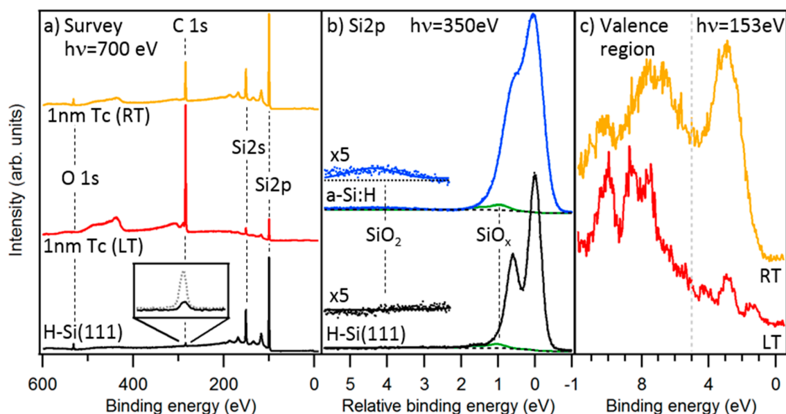
Figure 7. (a) XPS survey spectra of H-Si(111) before and after Tc deposition at LT as well as upon warming the Tc to room temperature (RT). (inset) Close-up of the C 1s region, including a spectrum of the substrate before annealing (gray dotted line). The annealed H-Si(111) substrate (720 K for 70 min, black) still features C 1s and O 1s intensity from substrate contamination not completely removed by the annealing. The red spectrum belongs to a Tc film of nominally 1 nm coverage deposited and measured at LT; the yellow spectrum was measured after warming up to room temperature (RT). Note (i) the increase of the C 1s signal upon Tc deposition and the corresponding decrease in Si 2p and Si 2s and (ii) the opposite trend upon raising the temperature to RT. (b) Si 2p region for H-Si(111) after annealing (black) and a-Si:H (blue). The binding energy scale is referenced to the Si 2p 3/2 peak maximum. Only small (~3%) substoichiometric oxide contributions (green) are observed. Traces of SiO 2 (~2%) can be resolved for a-Si:H, but not for H-Si(111). (c) Valence electron region for the same Tc film as in part a. For the cooled sample (red), the spectrum is dominated by the Tc molecular orbitals. Upon exposure to room temperature (yellow), the spectrum becomes dominated by the Si bands. The spectral regions above and below 5 eV (indicated by the vertical dotted line) were acquired with different statistics.
