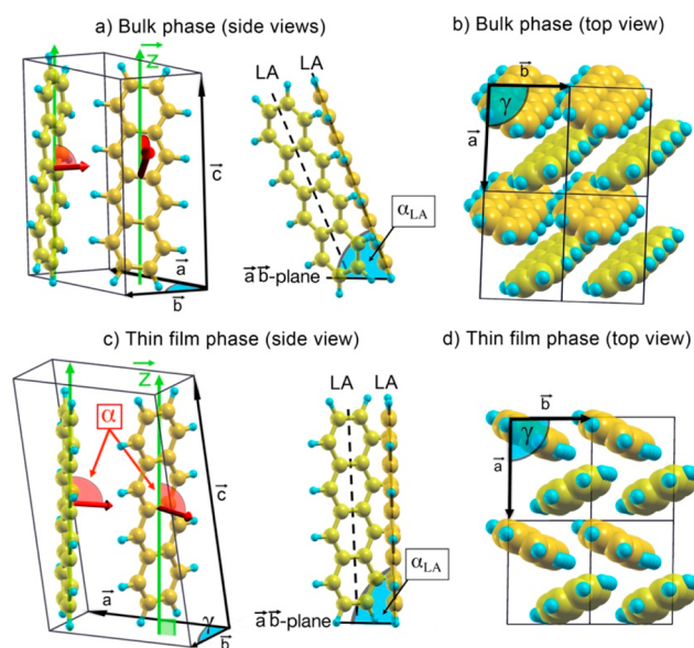
Figure 2. (a/c) Side and (b/d) top views for the experimentally determined structures of the tetracene bulk (Tc I, top) and thin film (Tc II, bottom) phases (structures published in refs 34 and 23), respectively. The parameters \bar{a} = 0.781 nm, \bar{b} = 0.603 nm and \gamma = 94.208^\circ ( \bar{a} = 0.756 nm, \bar{b} = 0.593 nm, and \gamma = 90.10^\circ ) define the lateral unit cell dimensions of the Tc I (Tc II) phase, whereby the unit cell of each phase includes two nonequivalent molecules. As a guide to the eyes, the carbon atoms in the nonequivalent Tc within a unit cell are shown in slightly different colors. It is a unique feature of the bulk phase that only one molecule is simply tilted, whereby the second molecule is tilted over the edge, so that one of the two bottom H atoms is considerably closer to the bottom of the unit cell (assumed to be the \bar{a}\bar{b} -plane); see also part a. With respect to this bottom \bar{a}\bar{b} -plane, the two nonequivalent molecules show almost the same orientation \alpha_{\text{LA}} for the long axis (LA) but differently rotated molecular planes. As a consequence, the average NEXAFS angle \alpha between the molecular plane normal (red arrows) and the surface normal ( \bar{z} -direction, green) deviates from \alpha_{\text{LA}} ( \alpha is always larger than \alpha_{\text{LA}} ). From the two phases, Tc II exhibits the denser morphology and the Tc molecules are more inclined with respect to the \bar{a}\bar{b} -plane ( \alpha_{\text{LA}} = 85.4^\circ instead of 69.48^\circ in Tc I).
