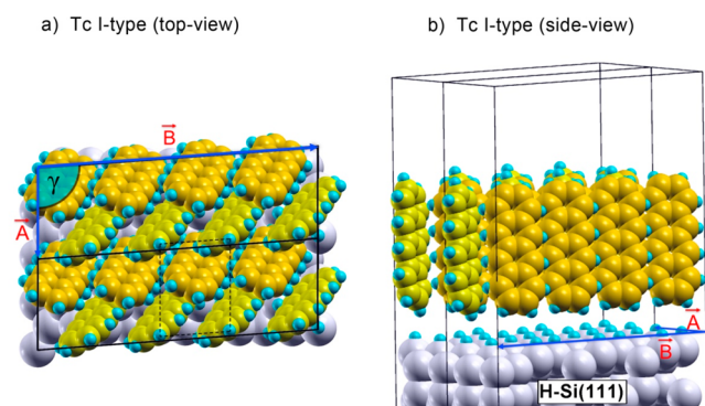
Figure 3. Modeling an ideal Tc monolayer (in LT regime): (a and b): top- and side-views, respectively, of the DFT-calculated most stable monolayers of Tc molecules at H–Si(111), denoted as Tc I-type monolayers. \vec{A} , \vec{B} , and the angle \gamma define the lateral supercell used to model the structure: \vec{A} = 0.772 nm, \vec{B} = 2.370 nm, and \gamma = 94.21^\circ resembling 1 \times 4 repetition of the crystalline unit cells (dashed lines). The corresponding epitaxy matrix is given by \begin{pmatrix} A_{\text{Tc I-type}} \\ B_{\text{Tc I-type}} \end{pmatrix} = \begin{pmatrix} 2 & -2 \\ 3 & 4 \end{pmatrix} \begin{pmatrix} \vec{x}_1 \\ \vec{x}_2 \end{pmatrix} , where \vec{x}_1 and \vec{x}_2 indicate the primitive vectors of the Si(111) surface. The carbon atoms of the two nonequivalent Tc molecules within a unit cell are shown in slightly different colors.
