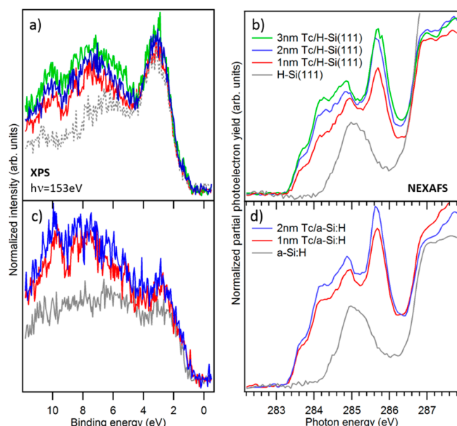
Figure 10. Experimental spectra for the Tc thickness series on H-Si(111), deposited and measured at T_{\text{sub}} = 265 K. (a) Valence electron region; (b) C K-edge NEXAFS. \theta was 20^\circ ( 30^\circ ) for the Tc films (the substrate-only spectrum). (c, d) Same as shown in parts a and b but for a-Si:H substrate. All spectra have been scaled so that the intensity of the substrate contribution stays identical, as determined via fits (for C K-edge NEXAFS) and linear combination of substrate- and Tc-dominated spectra (for the valence electron region). The substrate-only spectrum in part a was not measured but derived by subtracting the Tc-contribution from the 1 nm Tc/H-Si(111) spectrum.
