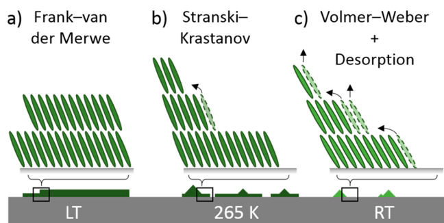
Figure 8. Schematic summary of Tc growth modes encountered in this work. (a) When Tc is deposited at LT, interlayer diffusion is completely absent, giving rise to Frank–van der Merwe (layer-by-layer) growth. (b) For Tc grown at 265 K, interlayer diffusion occurs predominantly for layers beyond the first monolayer, akin to Stranski–Krastanov growth. (c) At RT, also the first monolayer undergoes interlayer diffusion at high rates, leading to Volmer–Weber-type growth where 3D island formation consumes all Tc material. In addition, at RT significant Tc desorption takes place under UHV conditions.
