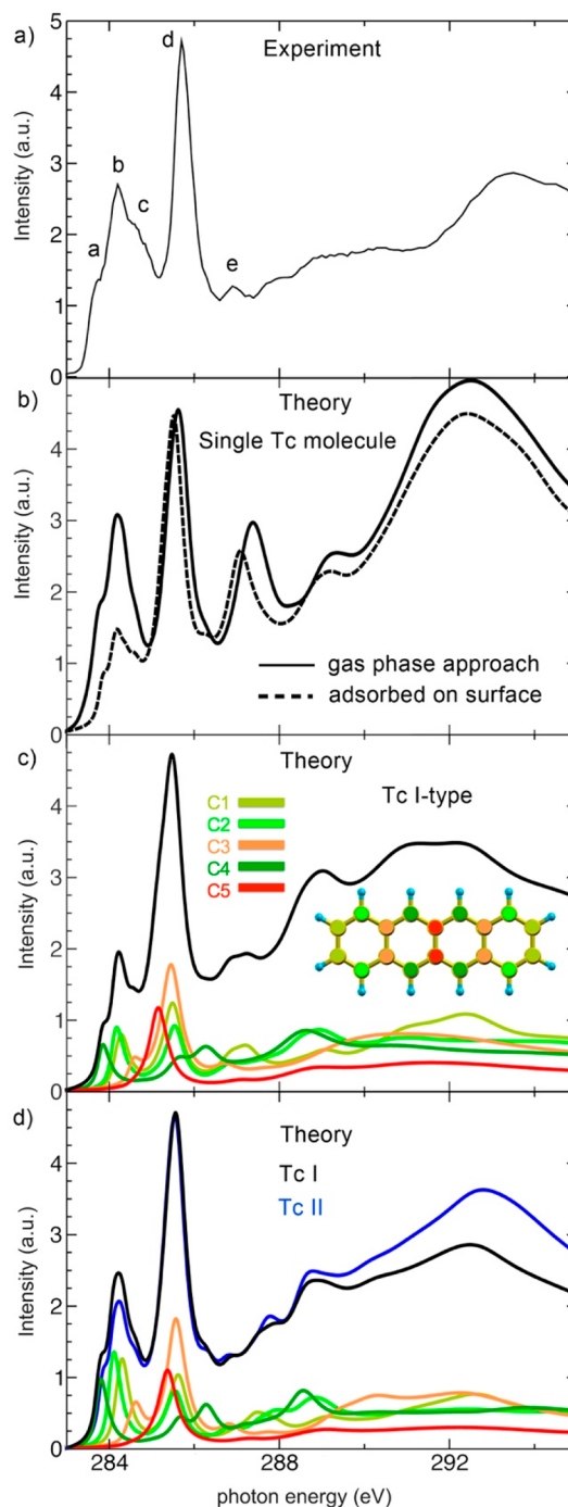
Figure 12. (a) Experimental NEXAFS C K-edge spectrum of the LT film, shown as an example at the incident angle \theta = 52.5^\circ . (b–d) DFT-calculated NEXAFS C K-edge spectrum for (b) a single Tc molecule in the gas phase/vacuum (solid line) and adsorbed on the surface (dashed), (c) the most stable Tc monolayer structure (Tc I-type shown in Figure 3), and (d) the crystalline bulk phase (black) and the crystalline thin-film phase (blue), respectively. All calculated spectra are also shown at incident angle \theta = 52.5^\circ . In parts c and d, the contributions of different C-atom types to the overall spectrum of the Tc I-type and Tc I (bulk) are also shown (bottom). (inset) Chemical structure of Tc that serves as a reference for the color code. The binding energies and the relative intensities of the first five characteristic resonances are shown in Table 3.
