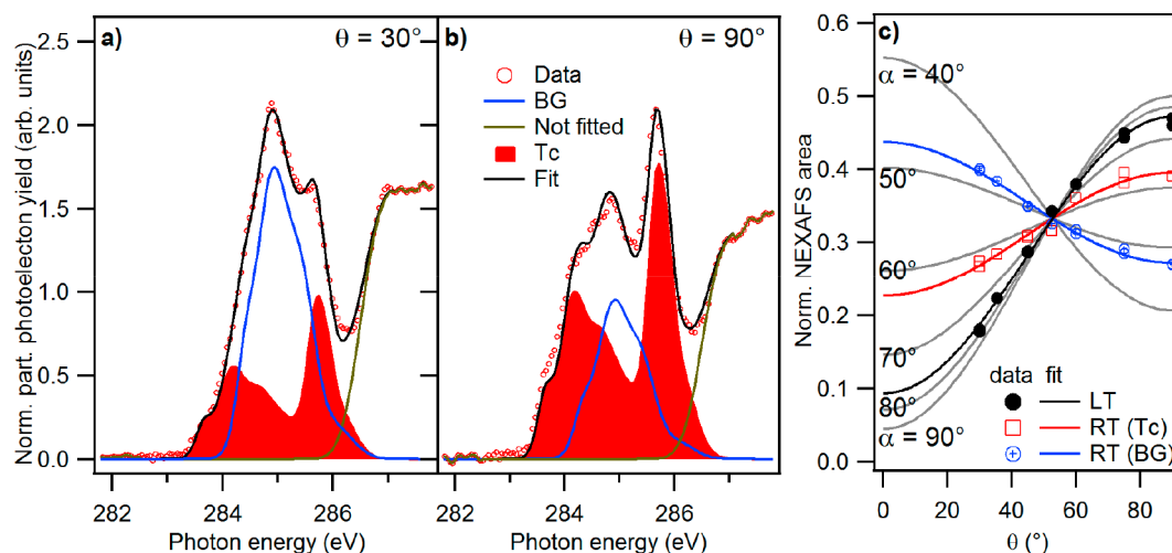
Figure 11. (a, b): NEXAFS C K-edge spectra measured at \theta = 30^\circ and 90^\circ X-ray incidence, respectively, for 1 nm Tc at H-Si(111) grown at LT and heated to RT. The fitted spectral contributions from Tc and the substrate are also shown. (c) \pi^* resonance intensities as a function of \theta for the following signals: Tc measured at LT, Tc measured at RT, the residual substrate carbon (background, BG) signal at RT. Data shown with fits according to eq 1, together with curves expected for some indicated \alpha .
