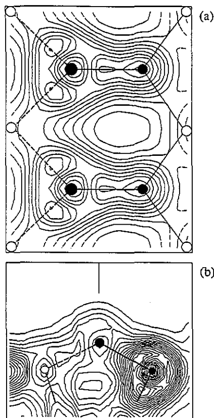
Figure 2. Contour plots of the total valence pseudocharge density for 0.5 ML with Al bonded to As (a) drawn along a horizontal plane 0.4 Å above the Al atoms and (b) drawn along a folded plane containing both the Al-As and Al-Ga bonds. The contours are spaced by 0.0025 and 0.005 e \times \text{Bohr}^{-3} , respectively.
