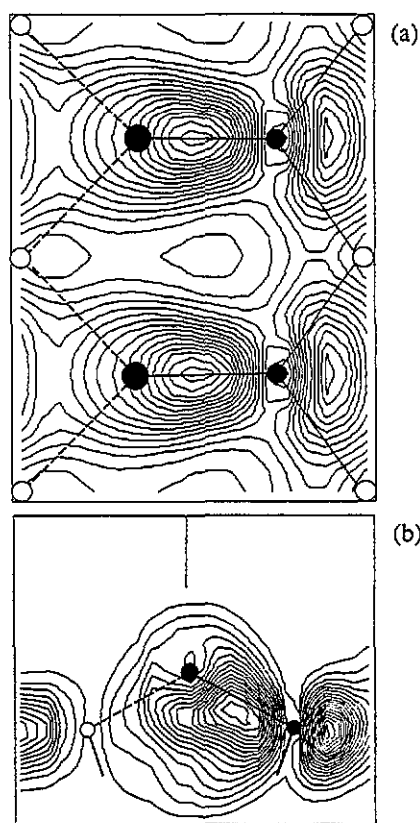
Figure 3. Orbital character of the half-occupied state pinning the Fermi level for 0.5 ML near X' (a) drawn along a horizontal plane 0.8 Å below the Al atoms and (b) drawn along a folded plane containing both the Al-As and Al-Ga bonding. The contours are spaced by 0.00025 e \times \text{Bohr}^{-3} .
