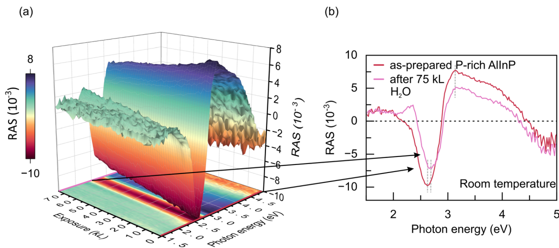
Fig. 1 (a) 3D color plot of in situ RAS measurement during exposure of 75 kL of water to P-rich AlInP (001) surface and (b) RA spectra measured at the beginning and end of the exposure. Red spectrum: as-prepared P-rich AlInP; pink spectrum: after 75 kL water exposure.
