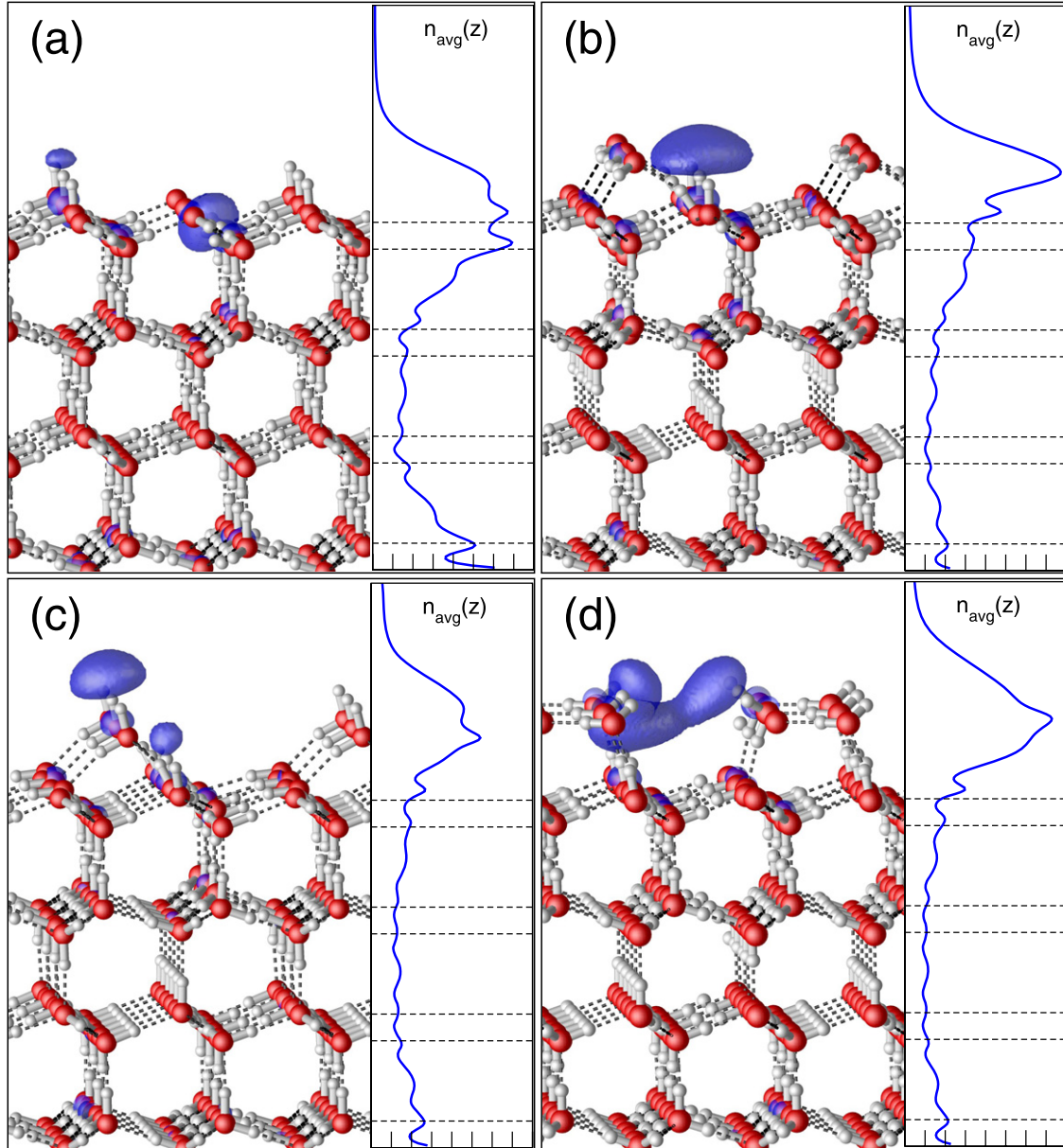
Figure 4. Excess electron density at various surface defect sites. \varrho_{\text{iso}} = 0.03 \text{ e } \text{\AA}^{-3} . (a) Surface vacancy, E_b = 1.11 \text{ eV} , (b) and (c) water monomer adsorbed surfaces, E_b = 0.08 \text{ eV} and -0.06 \text{ eV} , and (d) water dimer adsorbed surface, E_b = 0.04 \text{ eV} ; all per 2 \times 2 surface cell.
