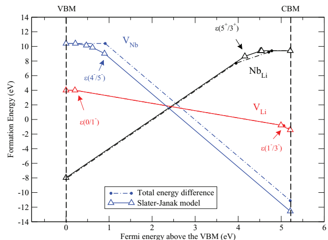
FIG. 4. Defect formation energies of \text{Nb}_{\text{Li}} , \text{V}_{\text{Li}} , and \text{V}_{\text{Nb}} in LN calculated with the Slater-Janak transition state model (solid lines) and by total-energy differences (dashed lines) as a function of Fermi energy.
