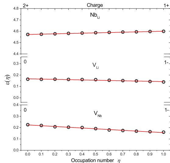
FIG. 3. Energy (in eV) of the highest occupied one-particle levels as a function of their occupation numbers for \text{Nb}_{\text{Li}}^{2+} , \text{V}_{\text{Li}}^- , and \text{V}_{\text{Nb}}^- in LN. The energy zero corresponds to the VBM.
