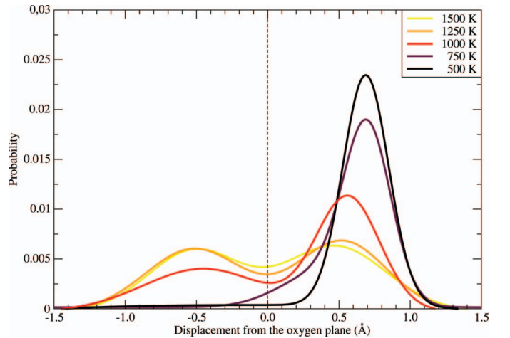
Fig. 2. Probability distribution of the parameter \Delta\text{Li} (representing the displacement of the Li ions from the oxygen planes) at different temperatures. The unimodal distribution at 500K (well below the Curie temperature) means that all of the Li ions are located above the oxygen planes, whereas the symmetric bimodal curve at 1500K (above the Curie temperature) indicates that the Li ions are randomly distributed above or below the oxygen planes, as expected for an order–disorder phase transition.
