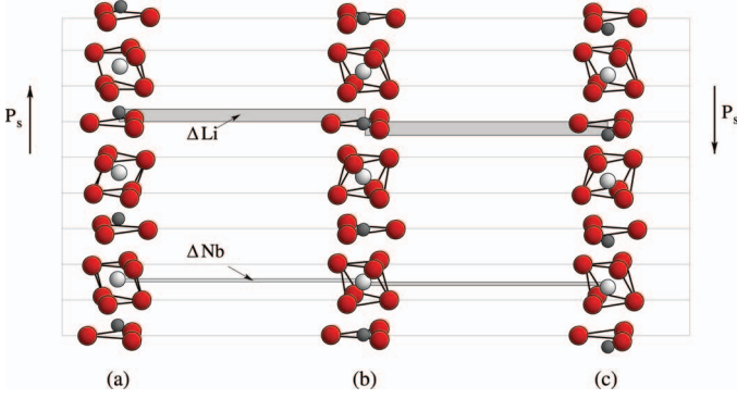
Fig. 1. Atomic structure of the (a) and (c) ferroelectric and (b) paraelectric phase of \text{LiNbO}_3 . The displacement of the Nb atoms (in white) from their positions in the paraelectric phase is labeled by \Delta\text{Nb} , whereas the displacement of the Li ions (in gray) from the oxygen planes is labeled by \Delta\text{Li} . Both displacements occur along the crystal c -axis.
