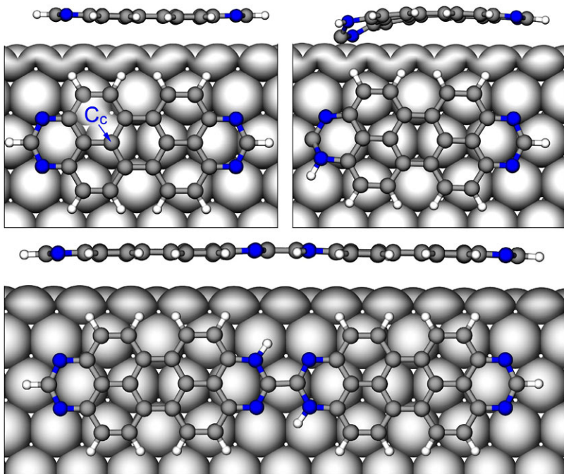
Fig. 1 Molecular model for the single TAPP molecule (left), the first tautomer TA1 (right) and the dimer adsorbed on the Cu(111) surface (bottom)
