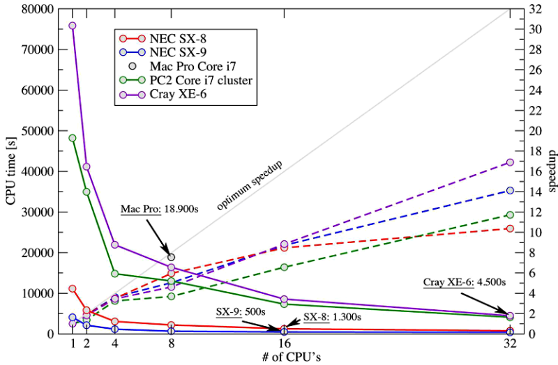
Fig. 2 CPU time and speedup for DFT calculations for the hexagon model of the Si(111)-In nanowire array containing around 200 atoms. The calculations were performed with the Stuttgart optimized VASP version on the HLRS NEC SX-8 and SX-9 machines. In comparison, we show data for the HLRS Cray XE6, a local Linux cluster (Intel Core i7, 24 Twin-nodes with 4 CPUs 2.5 GHz Quad Core Xeon each) and Mac Pro workstations (Intel Core i7)
