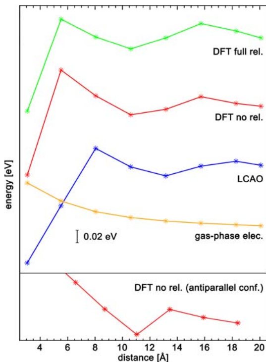
Fig. 5. Calculated modifications of the adsorption energy vs lateral spacing resulting from DFT-GGA calculations including structural relaxations, DFT-GGA calculations for frozen adsorbate and substrate, MO-LCAO calculations, and gas-phase dipole-dipole repulsion for the parallel molecular configuration are shown in the upper panel. The lower panel shows the corresponding DFT-GGA data for antiparallel molecular configuration (cf. Fig. 3)
