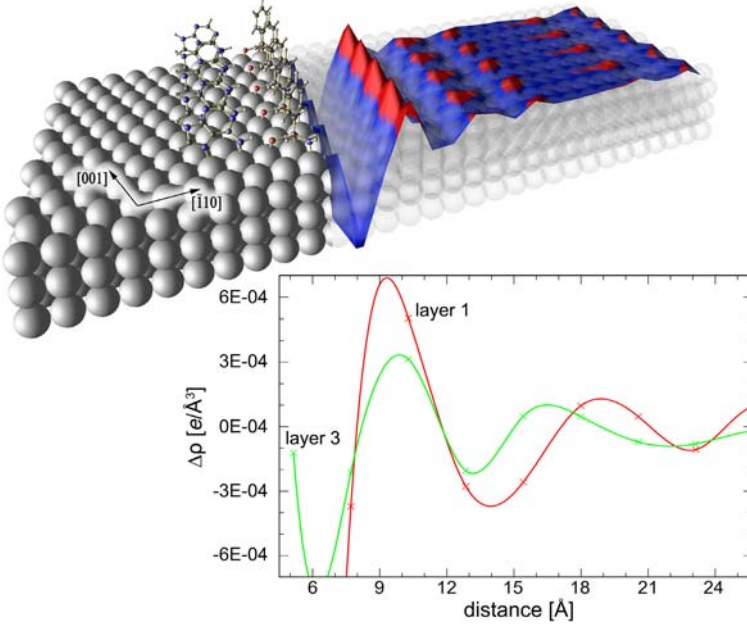
Fig. 4. Charge density difference of adenine and phenylglycine (1st row) adsorbed and clean Cu(110) surface. In the upper panel charge depletion and accumulation in the uppermost atomic layer are indicated blue and red, respectively. The lower panel shows the density differences in the first and third atomic layer vs the distance from the phenylglycine N atom along the [\bar{1}10] direction
