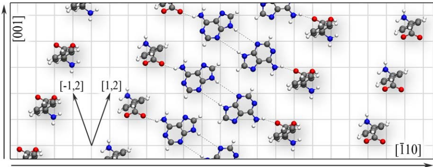
Fig. 1. Molecular model derived in Ref. [15] for phenylglycine co-adsorbed with adenine forming dimer rows along the [1,2] direction on Cu(110). Hydrogen bonds and the Cu(110) surface unit cells are indicated with dashed and gray lines, respectively
