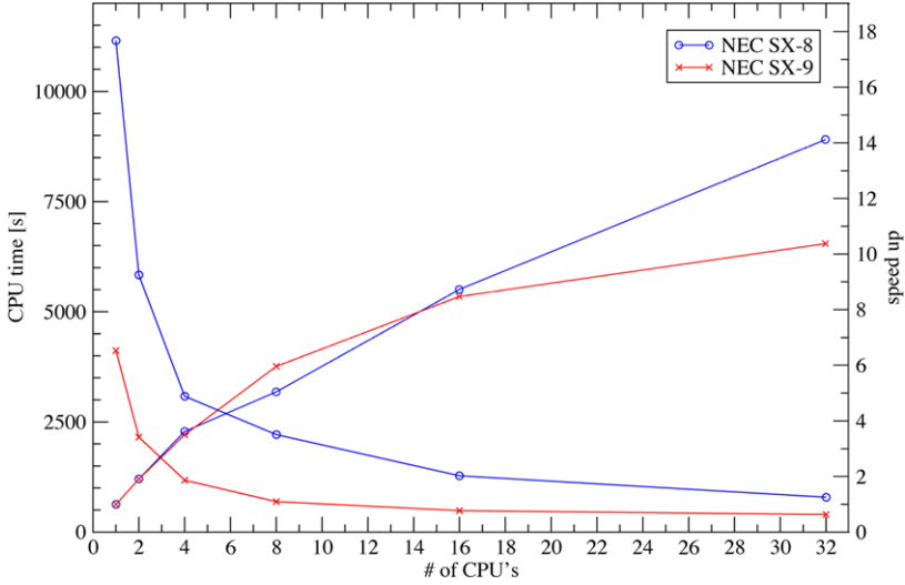
Fig. 2. Wall clock time and speedup for DFT calculations of a 200 atom cell used for surface modelling. The calculations were performed with the Stuttgart optimized VASP version on the HLRS NEC SX-8 and SX-9 machines
