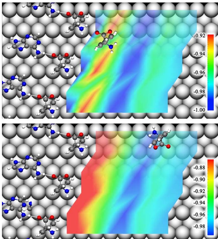
Fig. 3. Calculated adsorption energies (in eV, see text) of the 2nd row phenylglycine molecules for parallel (upper panel) and antiparallel (lower panel) orientation in the presence of pre-adsorbed adenine and phenylglycine. Thereby the leftmost atom of the 2nd row phenylglycine serves as molecular point of reference
