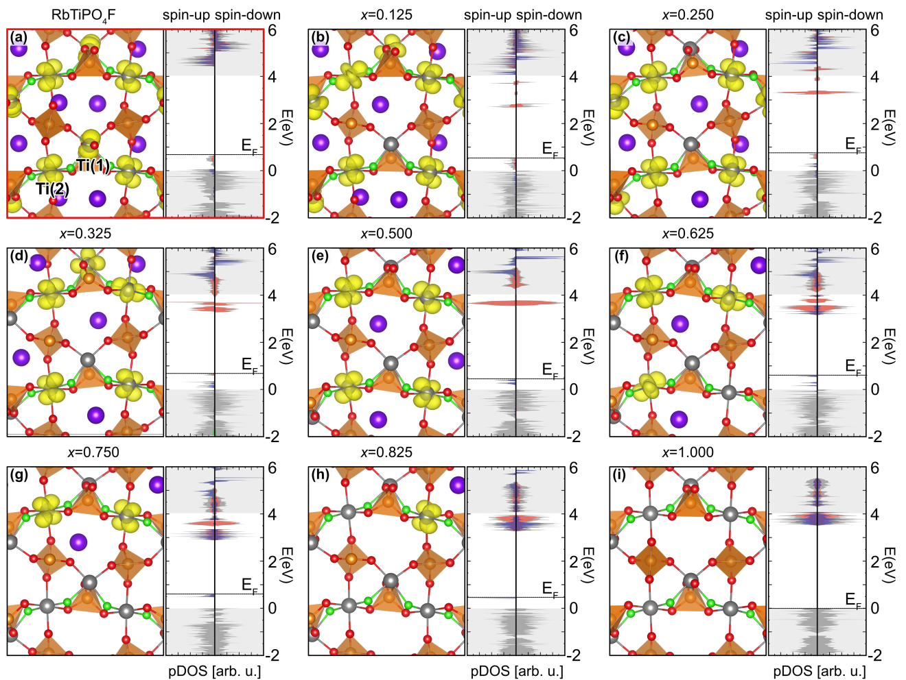
Figure 2. (a) Geometry (l.h.s.) and pDOS (r.h.s.) of the stoichiometric RTP:F unit cell after geometry relaxation. The Ti(1) and Ti(2) states are depicted in red and blue, respectively. Notably, they are clearly separated from each other. (b–i) Geometries and pDOS of \text{Rb}_{1-x}\text{TiPO}_4\text{F} after the deintercalation of different concentrations x = 0.125 – 1.000 of Rb. The yellow isosurfaces represent the spin-density difference of the spin-up and the spin-down channel, clearly showing the localization of the occupied defect states at the Ti sites and their consequent oxidation from \text{Ti}^{+3} to \text{Ti}^{+4} upon the deintercalation of Rb. Note that for x \leq 0.5 (i.e., structures (b–e)) only Ti(1) have been oxidized. E_F indicates the Fermi level position.
