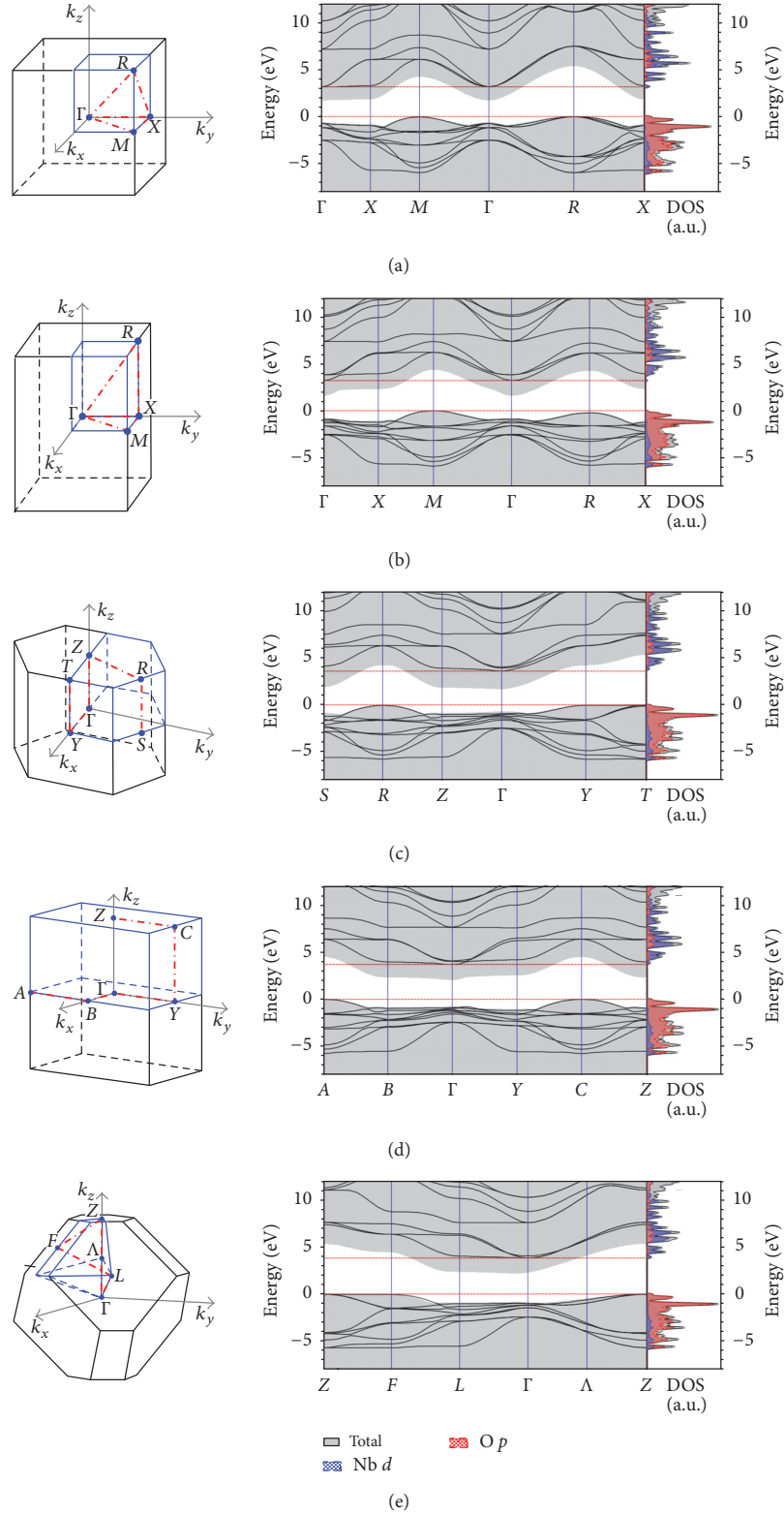
FIGURE 5: Band structures calculated with the HSE-30 functional for the cubic (a), tetragonal (b), orthorhombic (c), monoclinic (d), and rhombohedral (e) phases of \text{KNbO}_3 with corresponding densities of states (DOS) in arbitrary units. The grey-shaded areas indicate the PBE band structures for comparison, and the dashed horizontal lines mark the valence-band maxima and conduction-band minima. All band-structure calculations are based on structural data from PBESol (see Table 7). On the left-hand side, the chosen paths within the first Brillouin zone are indicated by thick dash-dotted lines.
