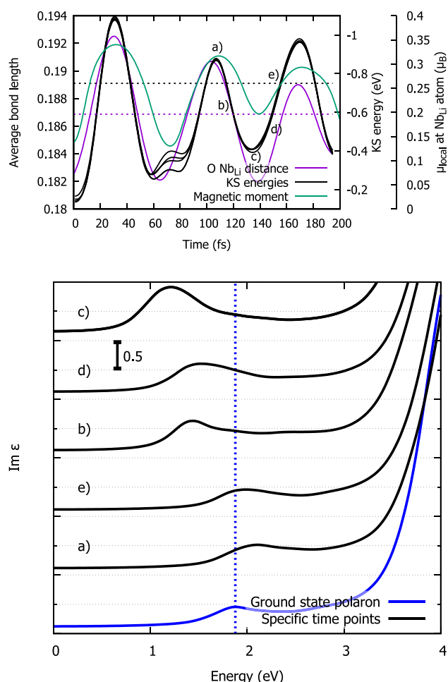
Fig. 3 (Top:) Evolution of the Kohn-Sham eigenvalues of the uppermost occupied electron state at four selected k points, average \text{Nb}_{\text{Li}}-\text{O} bond length (in units of the unit cell dimension), and \text{Nb}_{\text{Li}} local magnetic moment for a 200 K MD. Dashed lines mark the polaron ground state eigenvalues and O positions. (Bottom:) Imaginary part of the dielectric function ( zz component) calculated for snapshot structures at the times indicated in the top graph as well as for the ground state polaron. The vertical dashed line indicates the position of the ground state polaron peak
