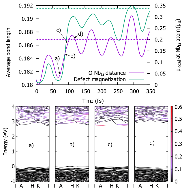
Fig. 2 (Top:) Evolution of the \text{Nb}_{\text{Li}} local magnetic moment and average \text{Nb}_{\text{Li}}\text{-O} bond length (in units of the unit cell dimension) for the same MD as shown in Fig. 1. Dashed lines mark the polaron ground state magnetic moment and O positions. (Bottom:) Polaron band structures for specific times, with colors indicating the electron localization
