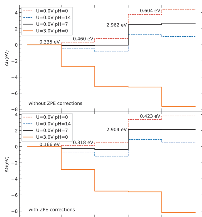
Figure 10. Comparison of the Gibbs free energy for the OER for different potentials and pH values. Bottom and top figures with and without ZPE energy term, respectively. Numbers represent the energy barriers for 0 pH and no potential.
