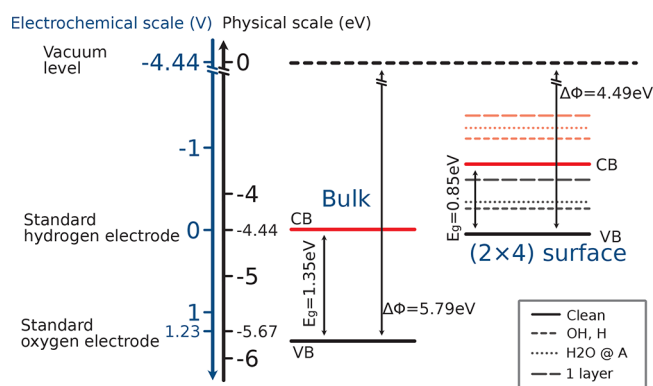
Figure 15. Band alignment of InP bulk and surface (calculated on the DFT-GGA level of theory) in relation to the water splitting redox potentials. Red/black lines depict CBs/VBs.
