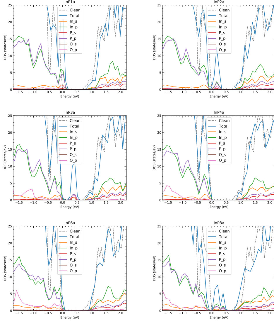
Figure S7: Calculated electron densities of states for oxidized mixed-dimer InP(001)(2 \times 4) surfaces in comparison to the clean surface. In addition to the total density, species-resolved s and p contributions are shown.
