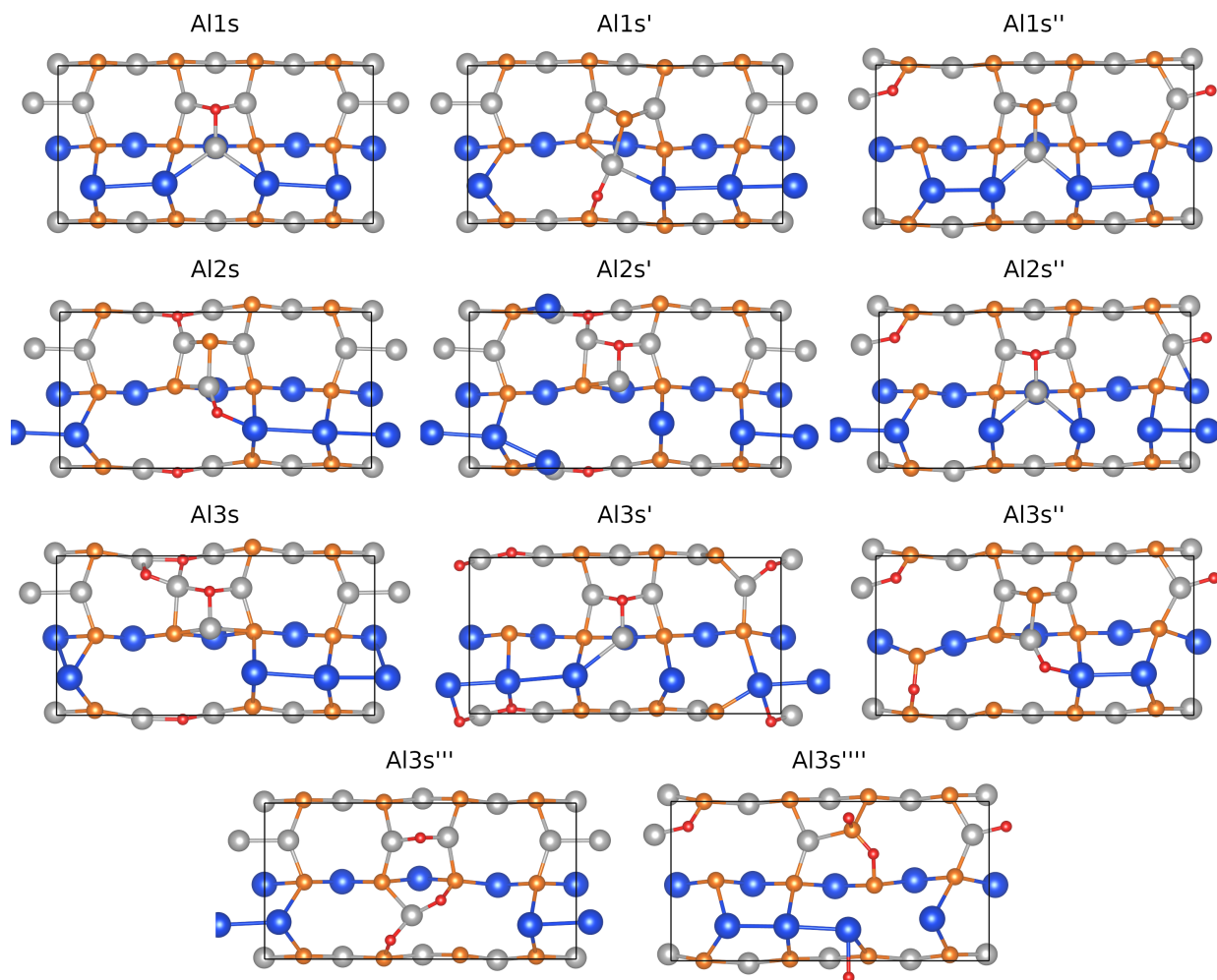
Figure S4: Top view of the most relevant models explored here for x oxygen substitution at the Al-P mixed dimer AlInP(001)(2×4) surface. The number in the notation indicates the number of substitute O atoms (s).
