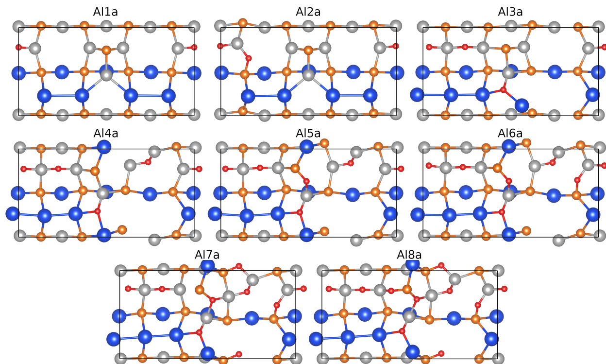
Figure S3: Top view of the models explored here for O adsorption at the Al-P mixed dimer AlInP(001)(2 \times 4) surface. The number in the notation indicates the number of O atoms adsorbed (a).
