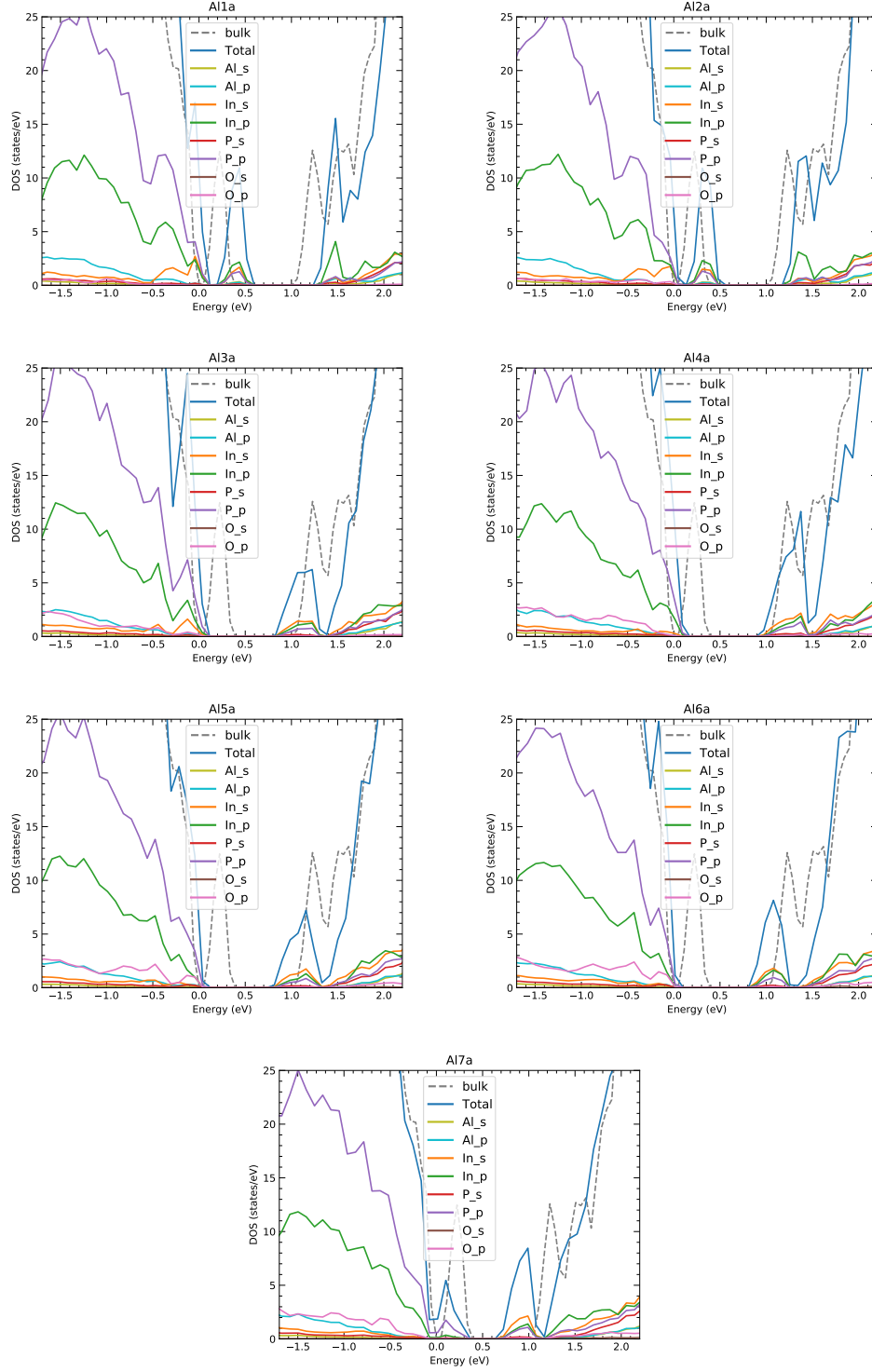
Figure S8: Calculated electron densities of states for oxidized Al-P mixed-dimer AlInP(001)(2 \times 4) surfaces in comparison to the clean surface. In addition to the total density, species-resolved s and p contributions are shown.
