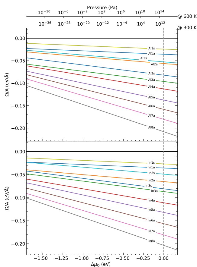
Figure 8. Surface grand-canonical potential vs oxygen chemical potential of the energetically most favored O adsorption and substitution geometries of AlInP(001). The O chemical potential on the bottom axis is given relative to molecular oxygen. The data calculated for the Al–P and In–P mixed-dimer structures are shown in the top and bottom panels, respectively.
