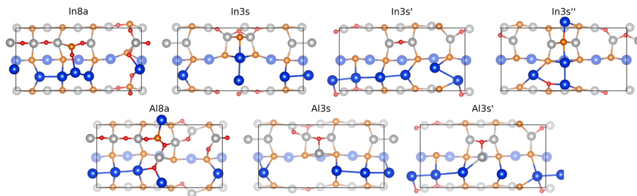
Figure 7. Energetically favorable O adsorption and substitution structures calculated for AlInP(001)( 2 \times 4 ) surfaces derived from the InP (top row) and AlP mixed-dimer models (bottom row), respectively. The complete set of relevant structures considered in the present work is shown in Figures S1–S6 in the SI.
