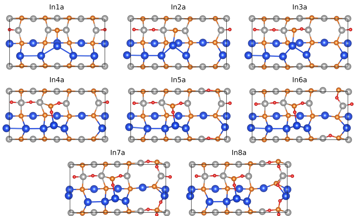
Figure S5: Top view of the models explored here for O adsorption at the In-P mixed dimer AlInP(001)(2×4) surface. The number in the notation indicates the number of O atoms adsorbed (a).
