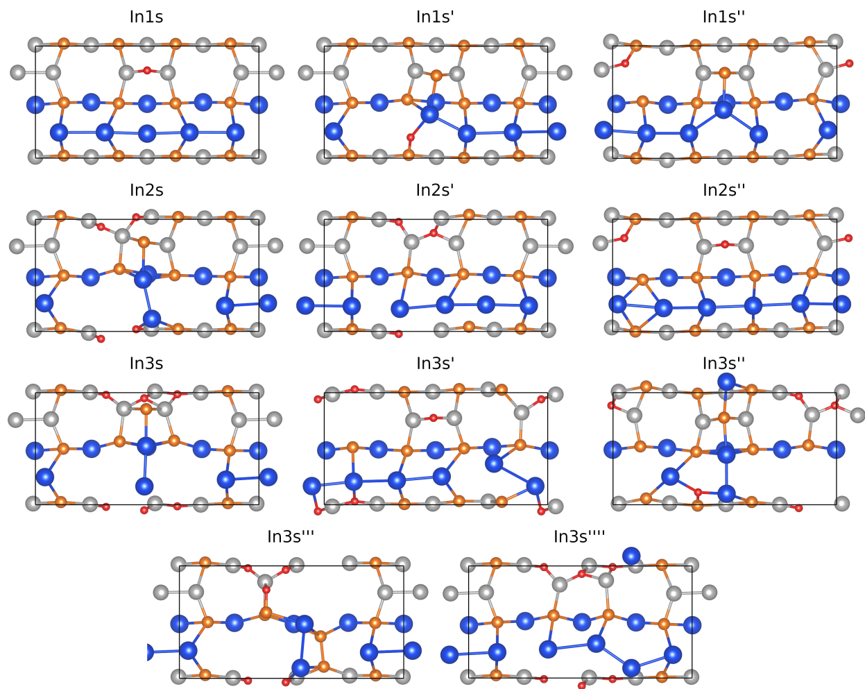
Figure S6: Top view of the most relevant models explored here for O substitution at the In-P mixed dimer AlInP(001)(2×4) surface. The number in the notation indicates the number of substitute O atoms (s).
