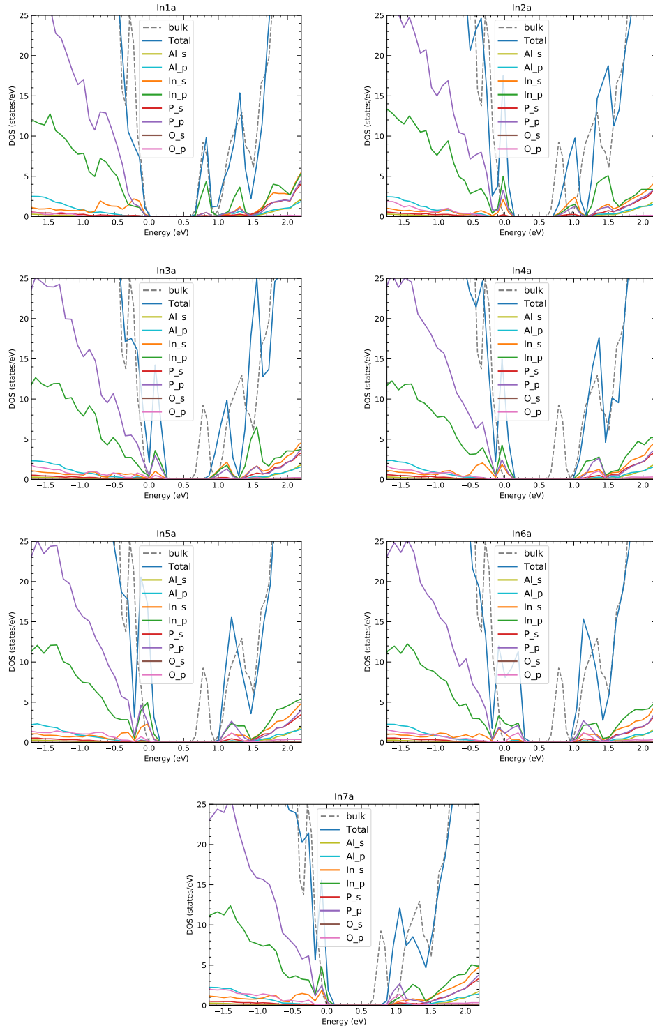
Figure S9: Calculated electron densities of states for oxidized In-P mixed-dimer AlInP(001)(2 \times 4) surfaces in comparison to the clean surface. In addition to the total density, species-resolved s and p contributions are shown.
