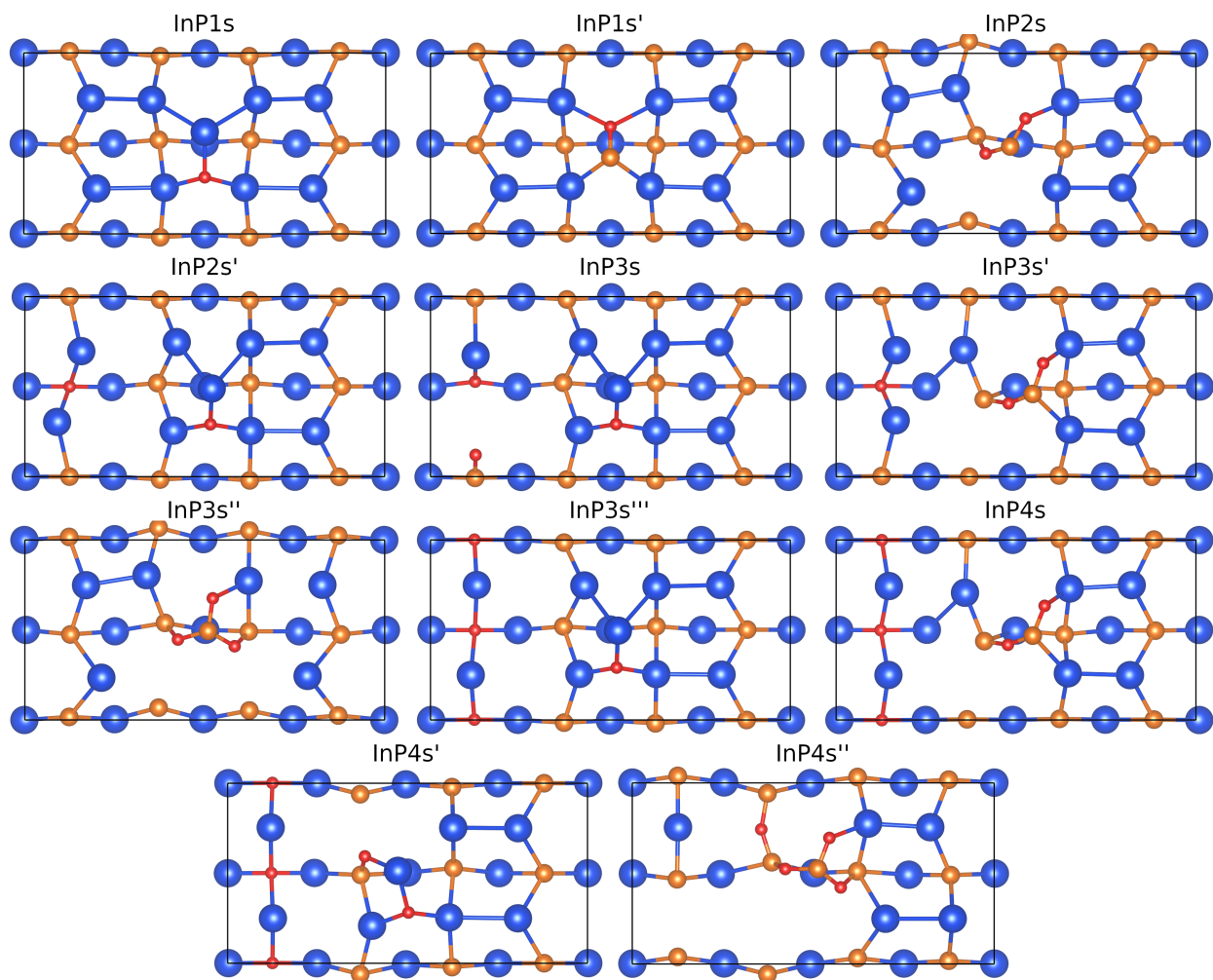
Figure S2: Top view of the most relevant models explored here for O substitution at the mixed-dimer InP(001)(2 \times 4) surface. The number in the notation indicates the number of substitute O atoms (s).
