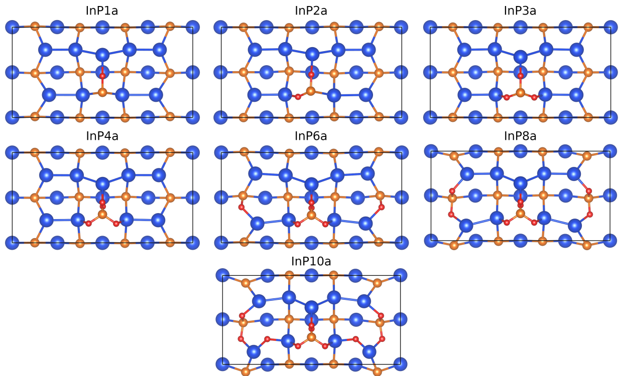
Figure S1: Top view of the models explored here for O adsorption at the mixed-dimer InP(001)( 2\times 4 ) surface. The number in the notation indicates the number of O atoms adsorbed (a).
